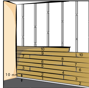
Pose horizontale
