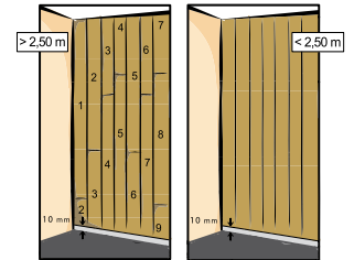
Pose verticale
